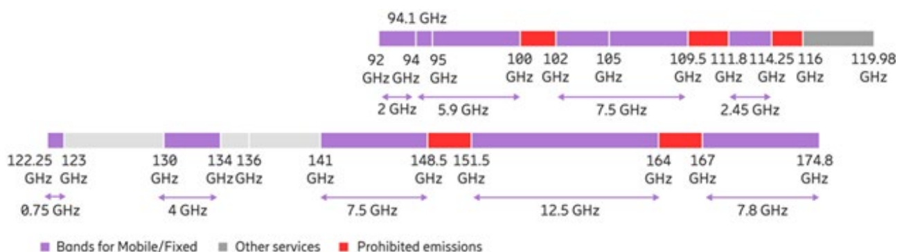
Figure 1. Frequency bands which are currently discussed for wide bandwidth 6G mobile communication (Source: https://www.ericsson.com/en/blog/2022/6/6g-spectrum-why-its-fundamental )
