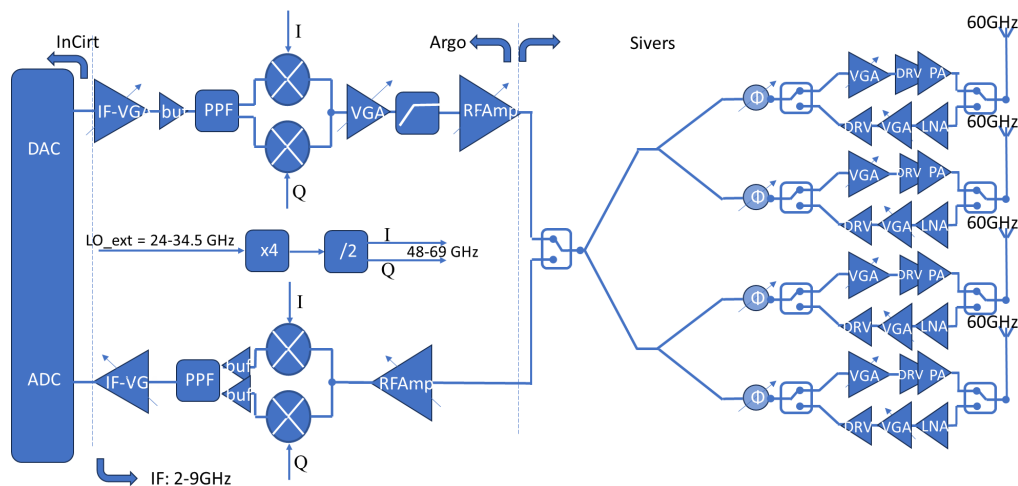
Figure 4. Proposed V-band TRx architecture (Source D1.1)
